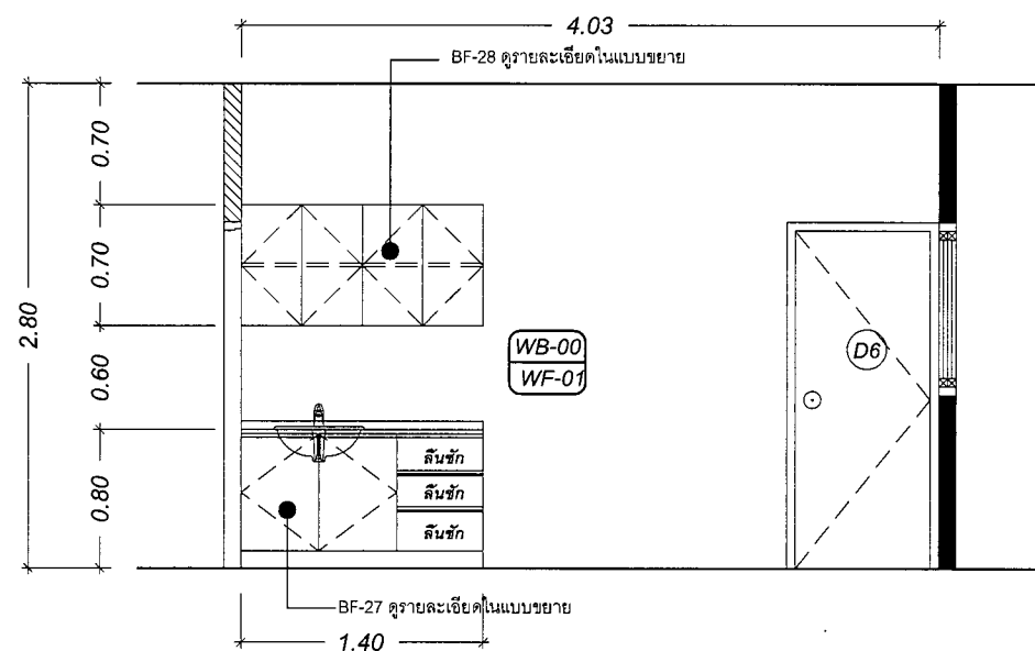
ELEVATION : A FIRST FLOOR SCALE 1:50
