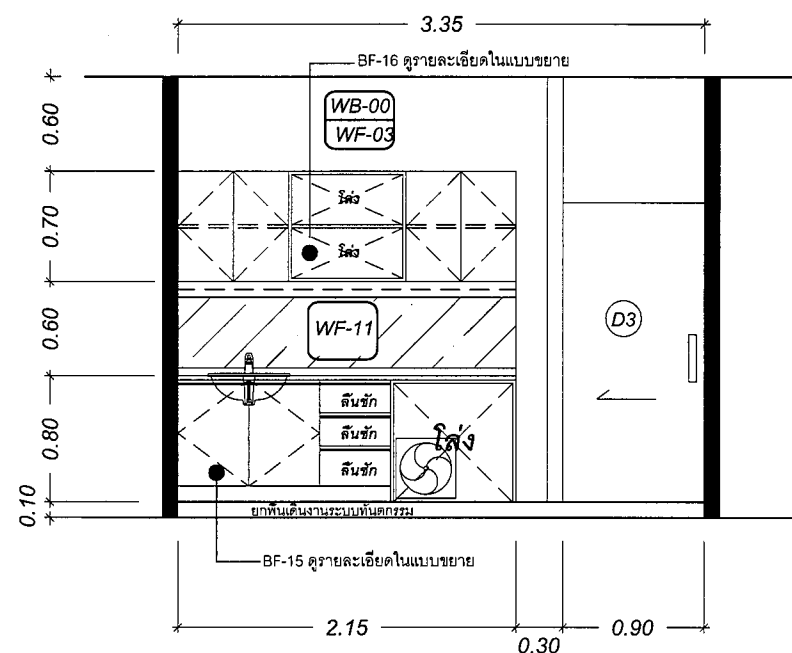
ELEVATION : A FIRST FLOOR SCALE 1:50
