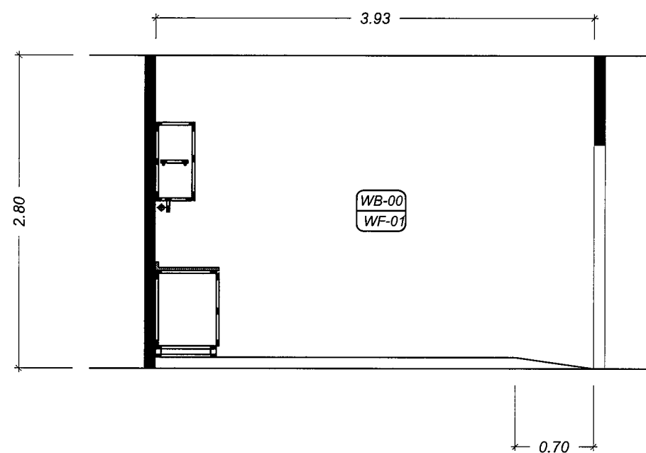
ELEVATION : C FIRST FLOOR SCALE 1:50
