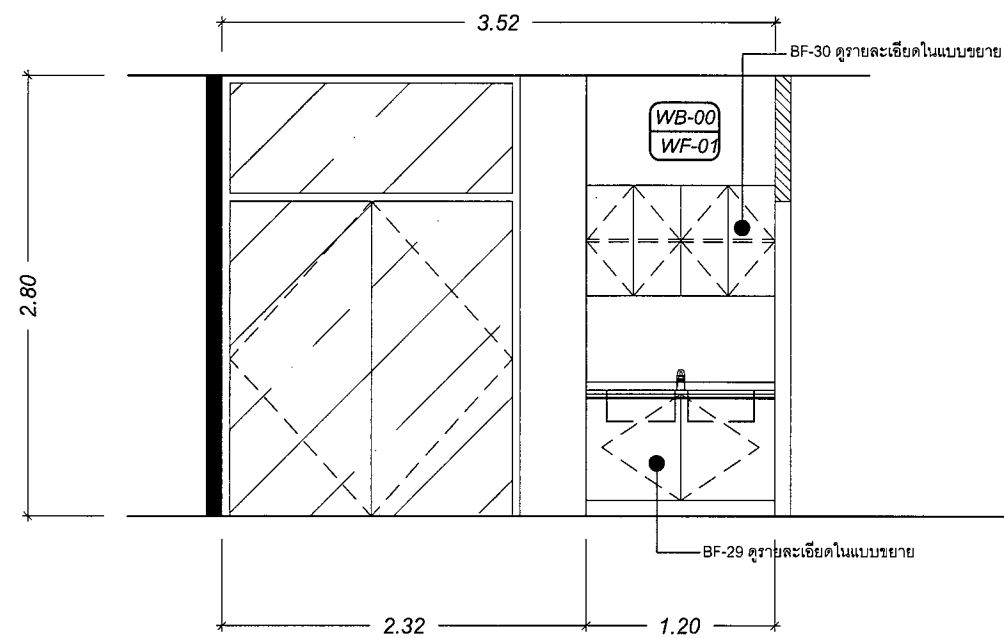
ELEVATION : A FIRST FLOOR SCALE 1:50
