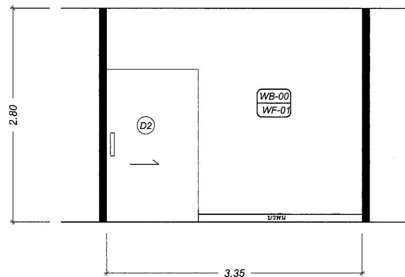
ELEVATION : B FIRST FLOOR SCALE 1:50
