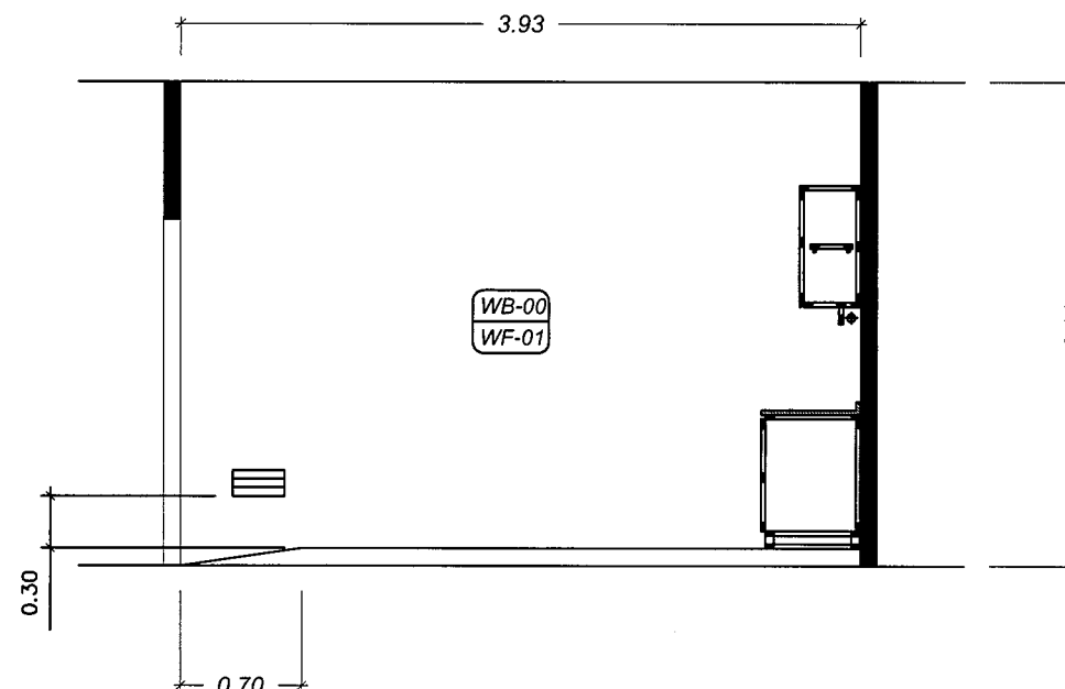
ELEVATION : D FIRST FLOOR SCALE 1:50
